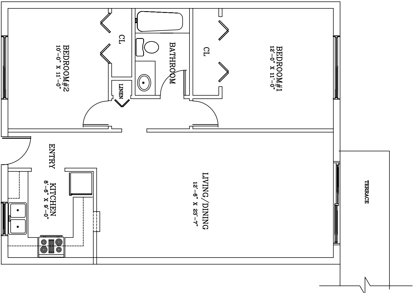
UNIT -2 BEDROOM
